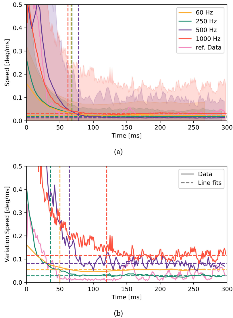
Figure 4.10: (a) Mean of the eye movement speed following a blink for the different frequencies of the stationary eye trackers in the data, including our reference data. We observe a steep decrease in speed after missing data appear, with values normalizing around 60 ms. (b) Variation of the eye movement speed following a blink for the different frequencies of the stationary eye trackers in the data, including our reference data. We observe a steep decrease in variation after missing data appear, normalizing around 120 ms. The vertical dashed lines represent the points identified as the first time the line crossed the fitted function plus epsilon for both (a) and (b).
