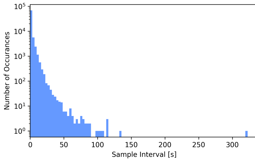
Figure 4.19: Illustration highlighting the interval (time between) of the logged samples over 8.8 ms (which should be the normal interval of a 125 Hz recording + allowance of 10% in variation).
