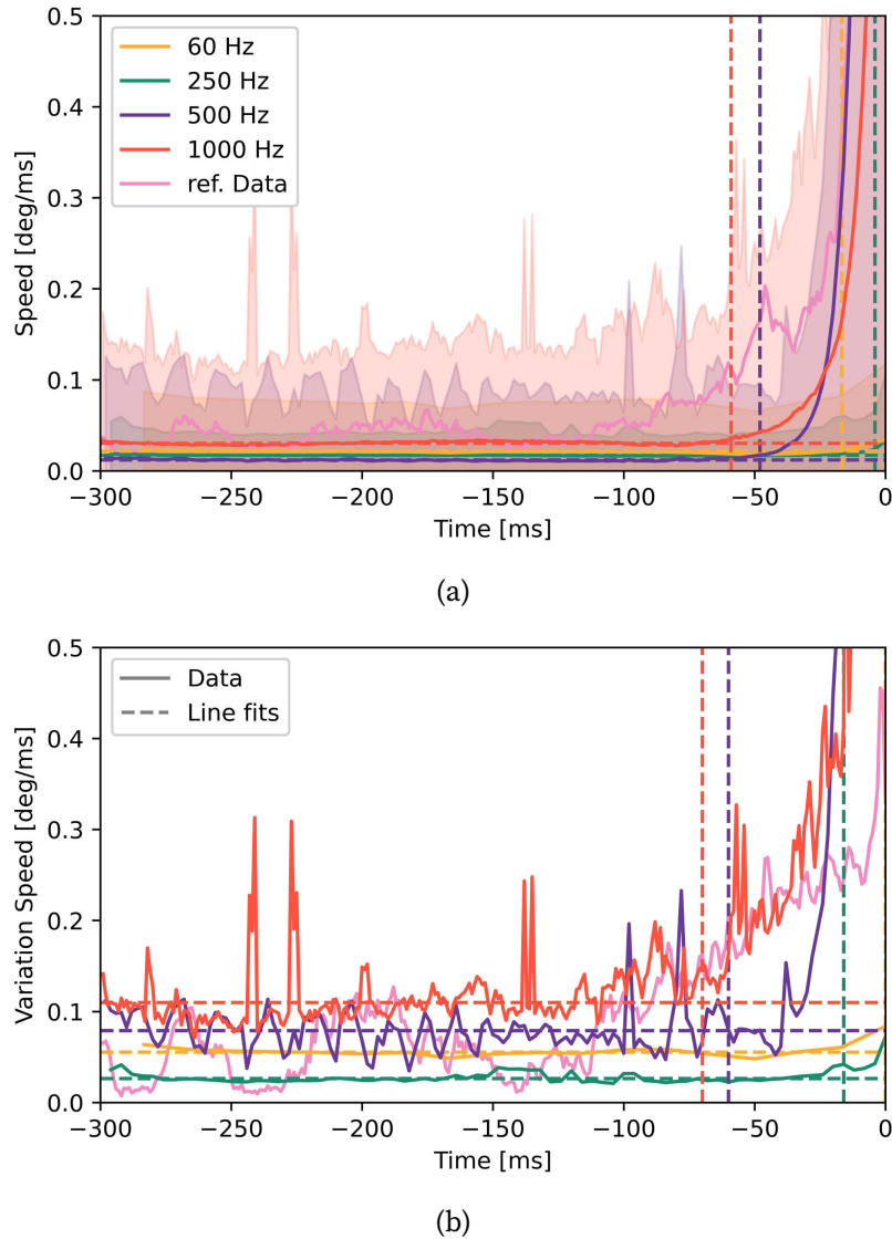
Figure 4.9: (a) Mean of the eye movement speed preceding a blink for the different frequencies of the stationary eye trackers in the data, including our reference data. We observe a steep increase in speed before missing data appears, around -60 ms. (b) Variation of the eye movement speed preceding a blink for the different frequencies of the stationary eye trackers in the data, including our reference data. We observe a steep increase in variation before missing data appears, around -70 ms. The vertical dashed lines represent the points identified as the first time the line crossed the fitted function plus epsilon for both (a) and (b).
