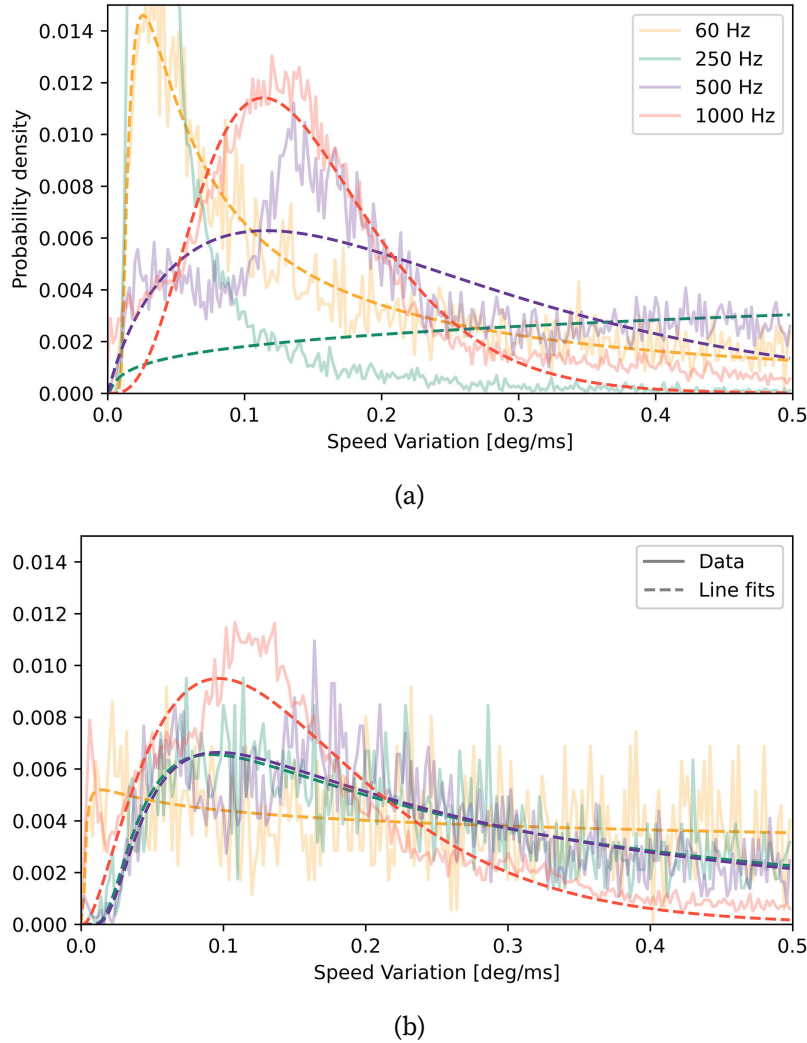
Figure 4.11: (a) Distribution of eye movement speed [deg/ms] from 50 ms preceding missing data for the different frequencies of the stationary eye trackers in the dataset. (b) Distribution of the variation of speed [deg/ms] from 50 ms following missing data for the different frequencies of the stationary eye trackers in the dataset. All dashed lines represent an inverse Gaussian distribution fitted to the data with an R^2 > 0.98 .
