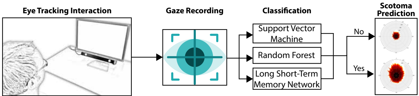
Figure 1: We investigate the computational cost and classification accuracy for predicting emerging CFL using eye-tracking data. We compare the efficiency of support vector machines, random forests, and long short-term memory networks to predict central field loss.
