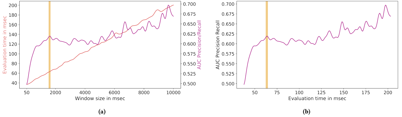
Figure 4: (a): Mean evaluation time plotted on the left-y-axis, mean AUC Precision-Recall plotted on the right-y-axis, the accompanying window size on the x-axis. The yellow line denotes the trade-off between the required window size and classification accuracy. A reasonable trade-off is achieved at ca. 1600 msec, since longer window sizes degrade the classification performance (e.g., due to loss of data through eye blinks). (b): Mean AUC Precision/Recall plotted on the y-axis and the accompanying evaluation time on the x-axis.
