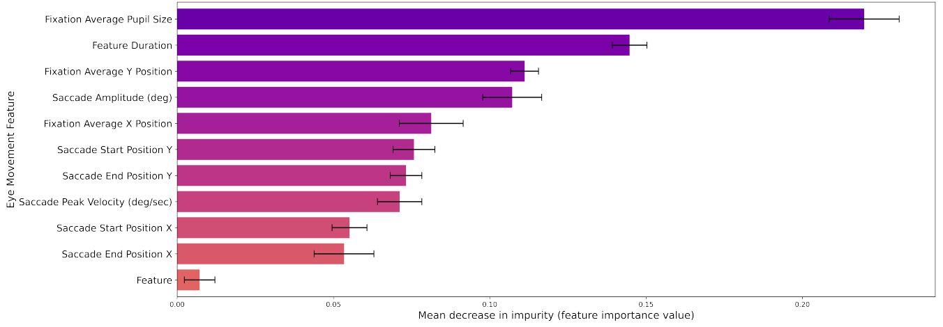
Figure 3: Feature importances measured by the mean decrease of Gini-impurity for the leave-one-participant-out nested cross-validation. The pupil size achieves the highest importance among all features.
